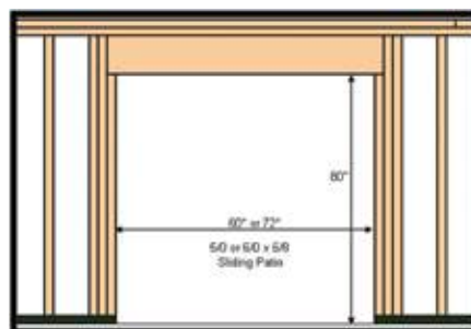
Rough Opening
